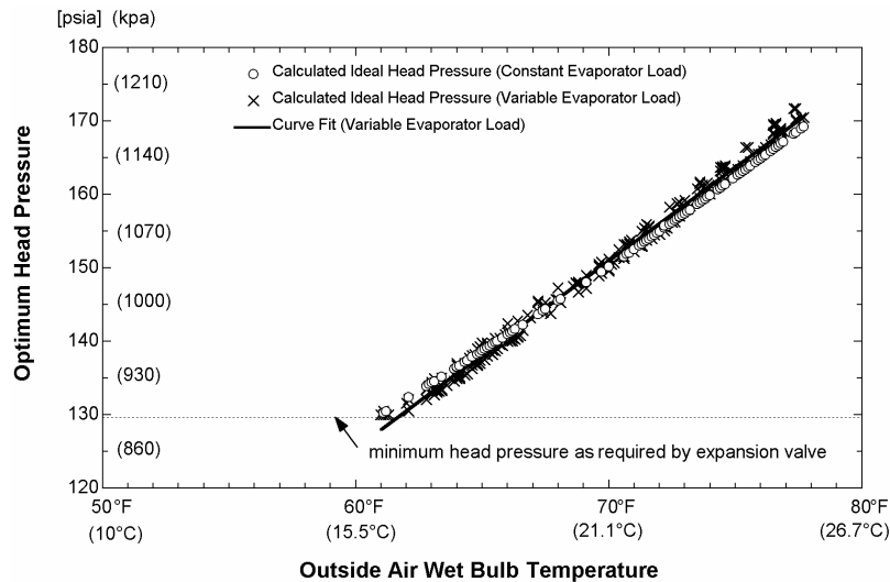
Figure 11: Optimum head pressure setpoints as a function of wet-bulb temperature.
