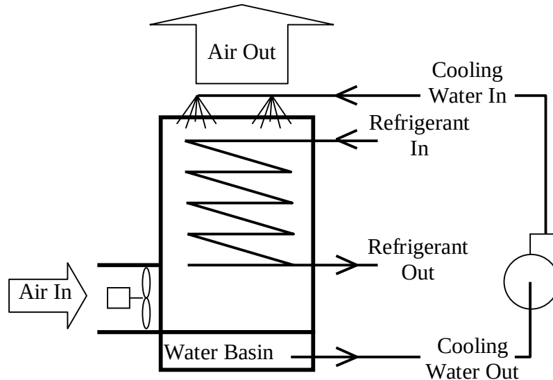
Figure 3: Schematic representation of the evaporative condenser.
