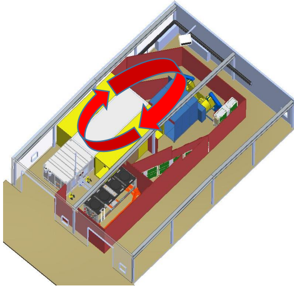
Figure 3: Model of Low Ambient Test Chamber for Air-Cooled Condensing Packaged System Testing
